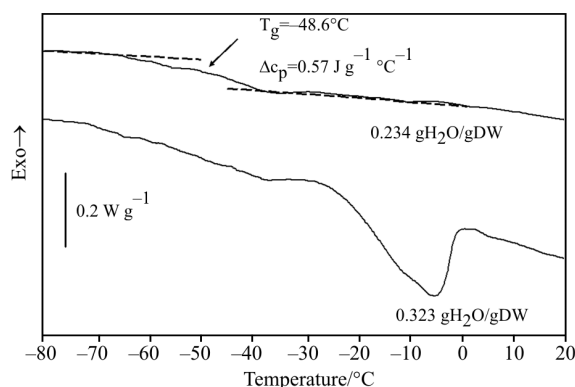
Fig. 2 Thermal characteristics of shoot tips dissected from bulblets of Allium sativum L. landrace Djambul 2 measured by DSC. The endothermic peak was measurable at water content 0.323 \text{ gH}_2\text{O/g dry mass} . After dehydration to the lower water content ( 0.234 \text{ gH}_2\text{O/g dry mass} ) the glass transition ( T_g ) with typical difference in a heat capacity occurred. The measurement were made during heating 10^{\circ}\text{C min}^{-1} (after previous cooling at 10^{\circ}\text{C min}^{-1} )
