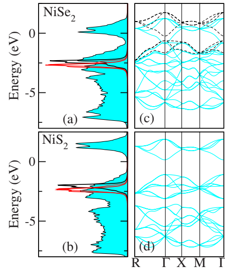
FIG. 6. (Color online) The bare S(Se)- p spectral densities and band structures. [(a) and (b)] The spectral densities in the left panel are obtained from a Wannier function Hamiltonian, while [(c) and (d)] the band structures in the middle panel are based on a linearized augmented plane-wave (LAPW) calculation with removed Ni-like basis functions. Dashed bands for \text{NiSe}_2 correspond to a reduced Se-Se distance.
