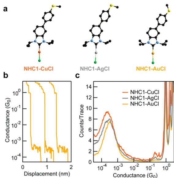
Figure 2. (a) Molecular structure of NHC1-MCl, as determined by SCXRD. Color code: black, C; blue, N; yellow, S; green, Cl; orange, Cu; gray, Ag; gold, Au. Hydrogens are omitted. (b) Sample conductance versus displacement traces of NHC1-AuCl, offset laterally for clarity. The plateau at \sim 3 \times 10^{-4} G_0 results from the single-molecule junction. (c) Logarithmically binned 1D conductance histograms (100 bins/decade) of NHC1-MCl junctions, each composed of at least 2000 traces without data selection. All measurements are in PC at a tip bias of -720 mV.
