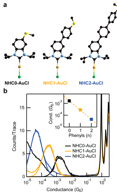
Figure 3. (a) Molecular structure of NHC n -AuCl ( n = 0, 1, \text{ and } 2 ), as determined by SCXRD. Note that the structure for NHC1-AuCl is repeated from Figure 2a for completeness. (b) Logarithmically binned 1D conductance histograms (100 bins/decade) of NHC n -AuCl, each composed of at least 2000 traces obtained without data selection. All measurements are performed in PC at a tip bias of -360 mV. (Inset) Semilogarithmic plot of the conductance histogram peak value as a function of the number of phenylene units in the backbone of NHC n -AuCl.
