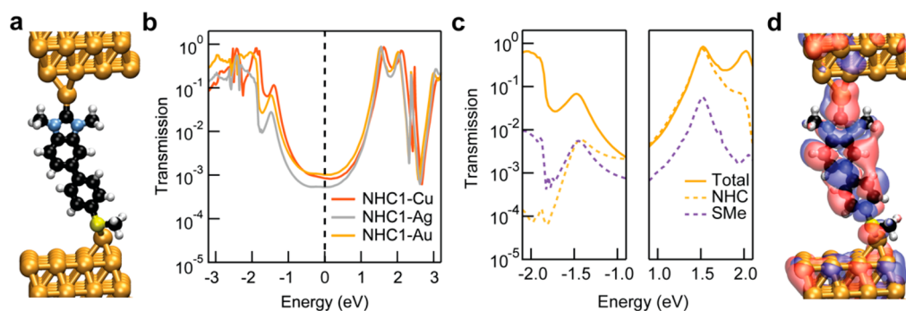
Figure 4. (a) Modeled structure of NHC1–Au junction. (b) Transmission function of NHC1–M junctions. (c) Projection of the electronic coupling matrices at the NHC and SMe contacts for the NHC1–Au junction onto the highest occupied molecular orbital (HOMO) (left) and lowest unoccupied molecular orbital (LUMO) (right). (d) Real-space representation of the most conducting transmission eigenchannel of NHC1–Au junction at the LUMO energy.
